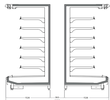
If Glint V3 1120 run cabinets are positioned back to back
