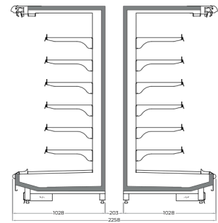
If Glint V3 950 / 1020 run cabinets are positioned back to back
