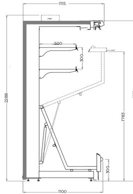
GLINT V3 2200 LIFT UP
