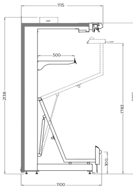
GLINT V3 2050 LIFT UP
