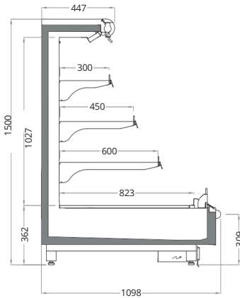
IRIS V3 1100 HI500 Length mm | 1250 | 1875 | 2500 | 3750 | HC:2136
