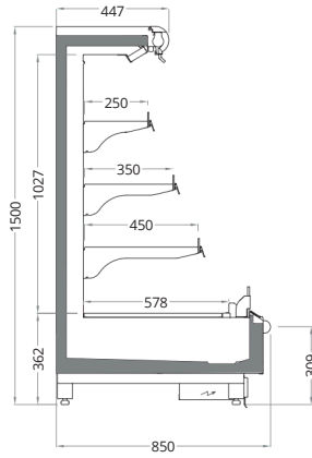
IRIS V3 850 HI500 Length mm | 1250 | 1875 | 2500 | 3750 | HC:1660
