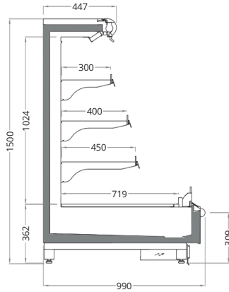
IRIS V3 1000 HI500 Length mm | 1250 | 1875 | 2500 | 3750 | HC:2136
