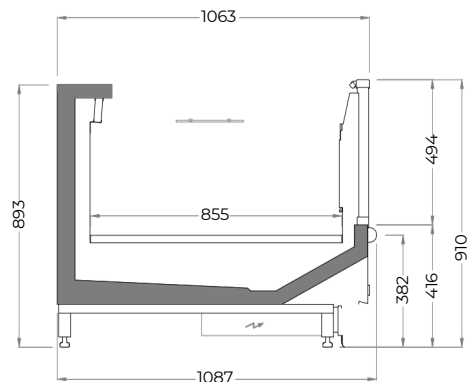
KRYOS WALL w/o LIDS
