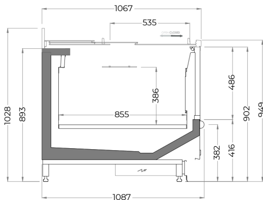
KRYOS WALL with LIDS
