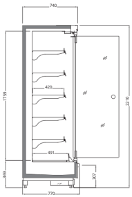
VECTO V3 2200 / 770 With Single Glass Doors
