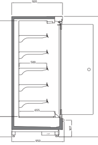
VECTO V3 2200 / 950 With Single Glass Doors
