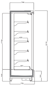
VECTO V3 2200 / 770 With Double Glass Sliding Doors
