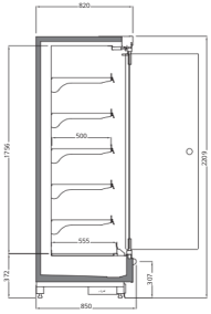
VECTO V3 2200 / 850 With Single Glass Doors
