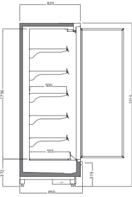
VECTO V3 2200 / 850 With Double Glass Doors
