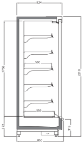
VECTO V3 2200 / 850 With Double Glass Sliding Doors
