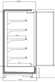
VECTO V3 2200 / 1090 With Double Glass Doors
