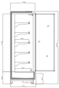
VECTO V3 2200 / 770 With Double Glass Doors
