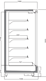
VECTO V3 2200 / 1090 With Double Glass Sliding Doors
