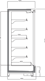
VECTO V3 2200 / 950 With Double Glass Sliding Doors
