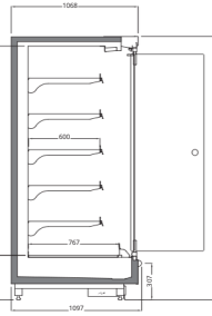
VECTO V3 2200 / 1090 With Single Glass Doors
