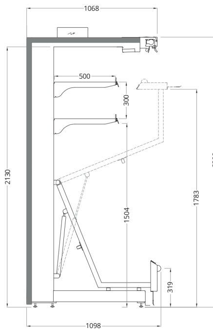
VECTO V3 2200 LIFT UP
