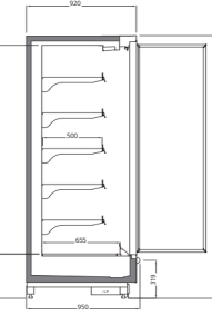
VECTO V3 2200 / 950 With Double Glass Doors
