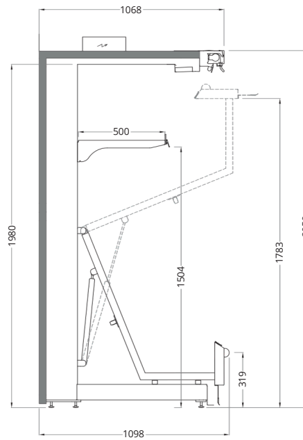
VECTO V3 2050 LIFT UP
