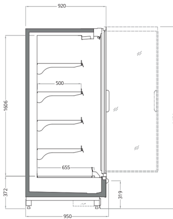
VECTO SKY 2050 / 950 / 320 Length mm | 1250 | 1875 | 2500 | 3750 | HC:1875
