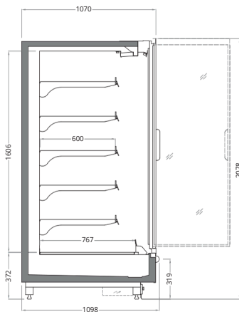
VECTO SKY 2050 / 1090 / 320 Length mm | 1250 | 1875 | 2500 | 3750 | HC:2136
