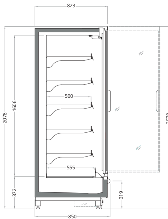
VECTO SKY 2050 / 850 / 320 Length mm | 1250 | 1875 | 2500 | 3750 | HC:1660
