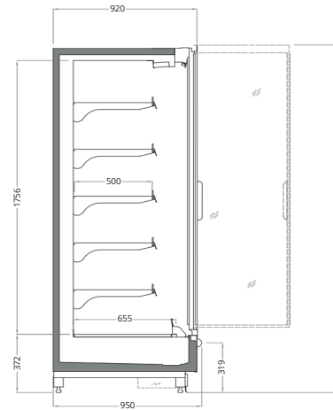
VECTO SKY 2200 / 950 / 320 Length mm | 1250 | 1875 | 2500 | 3750 | HC:1875
