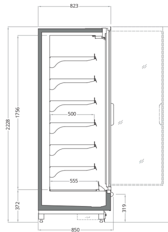
VECTO SKY 2200 / 850 / 320 Length mm | 1250 | 1875 | 2500 | 3750 | HC:1660
