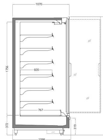
VECTO SKY 2200 / 1090 / 320 Length mm | 1250 | 1875 | 2500 | 3750 | HC:2136
